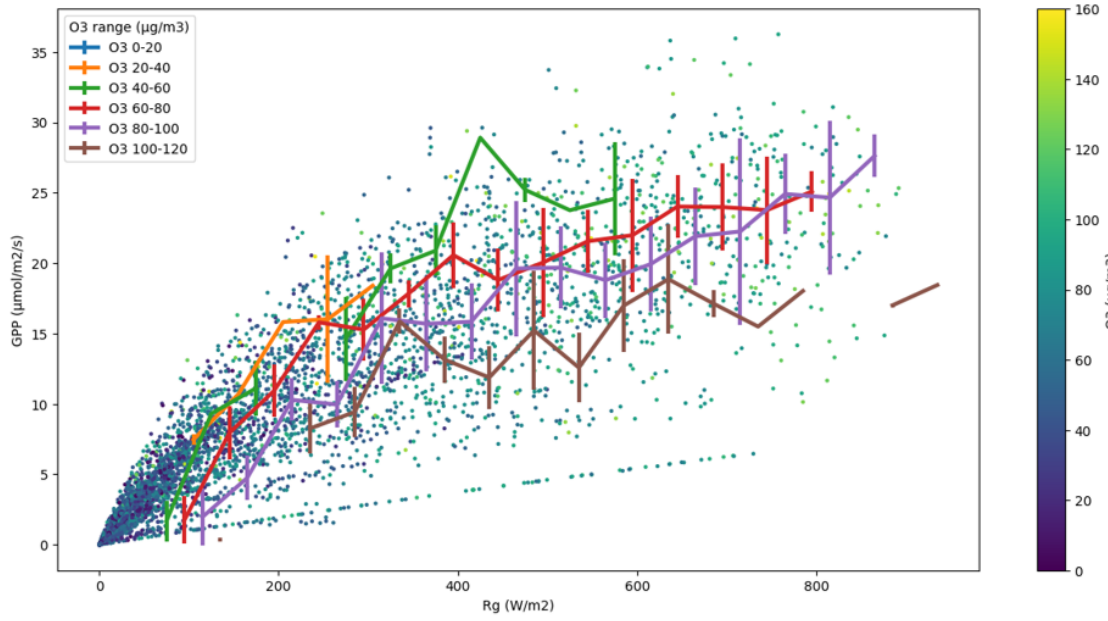
Figure 2.2: LRCs for different [O_3] ranges under defined conditions
