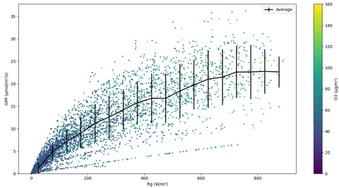
Figure 2.1: LRC from all GPP datapoints
